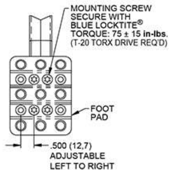
FOOT PAD DETAIL
